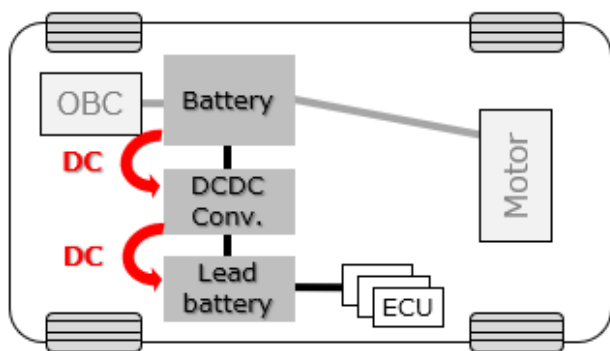
Figure 2: DC/DC converter work in EV
