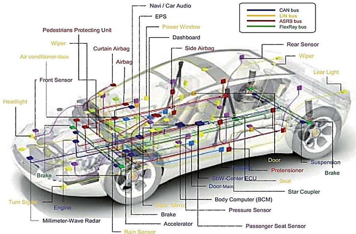
Figure 18: visual representation of CAN-BUS networks and communication protocols
