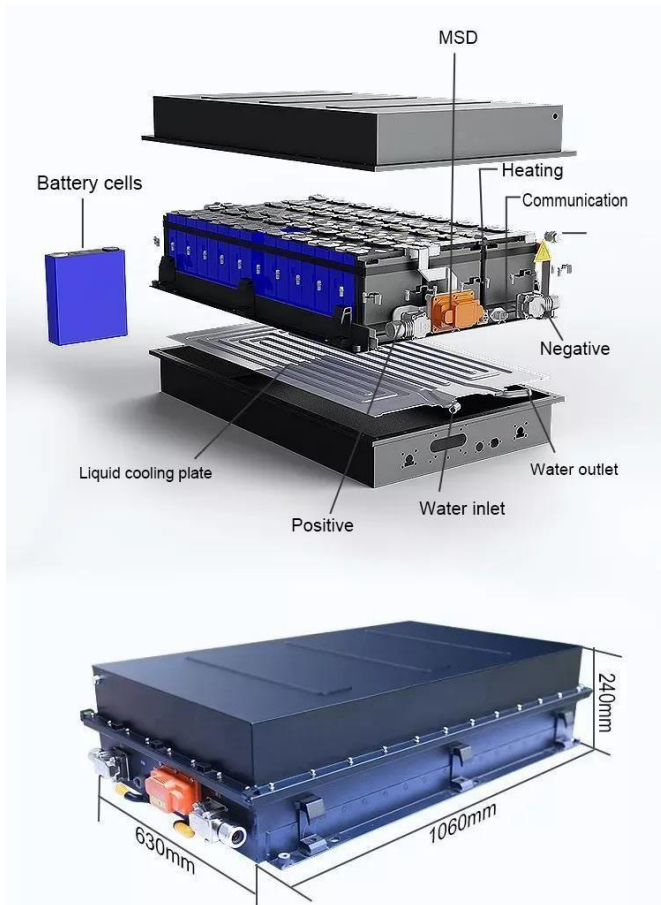
Figure 24: Battery components and measures
