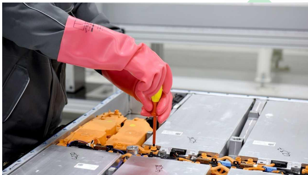
Figure 32: Battery dismantling process
