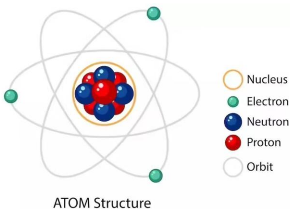
Figure 11: The structure of an atom
