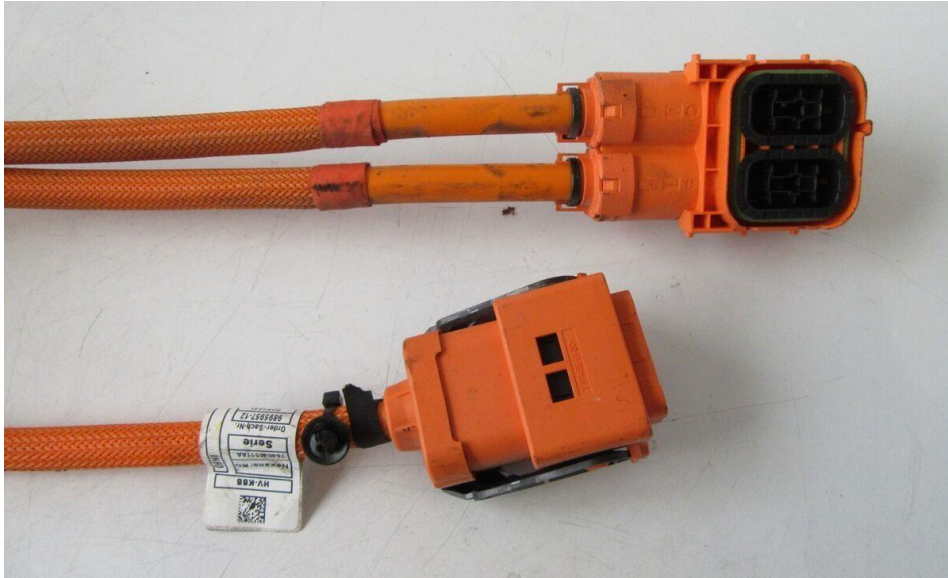
Figure 20: Orange cable
