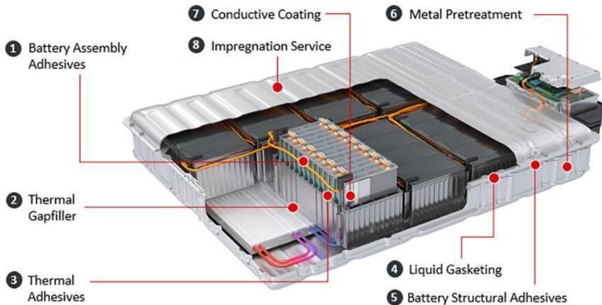
Figure 25: Battery pack components
