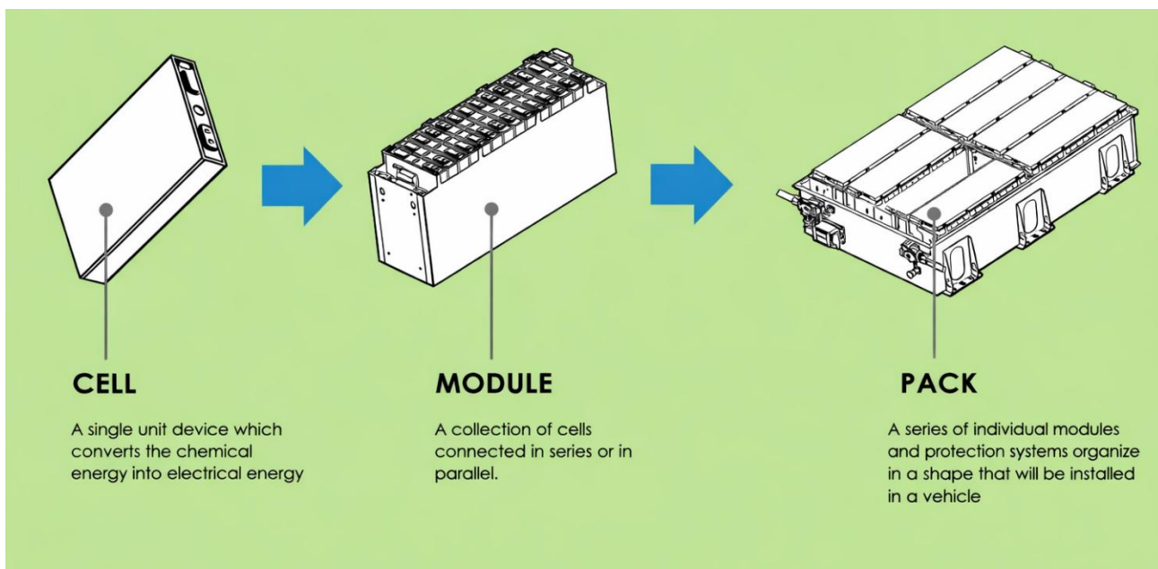
Figure 33: Schematic of an EV battery pack, composed of cells grouped into modules, with a BMS monitoring the cells and controlling contactors
