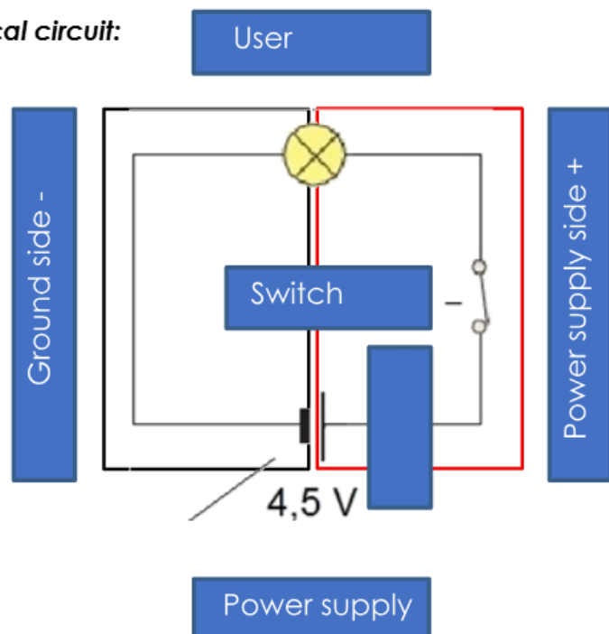
Figure 10: The basic components of an electrical circuit
