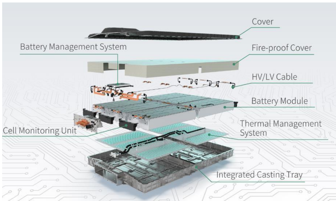
Figure 30: Battery assembly
