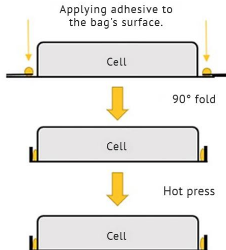
19. Steps for folding cell edges using adhesive
