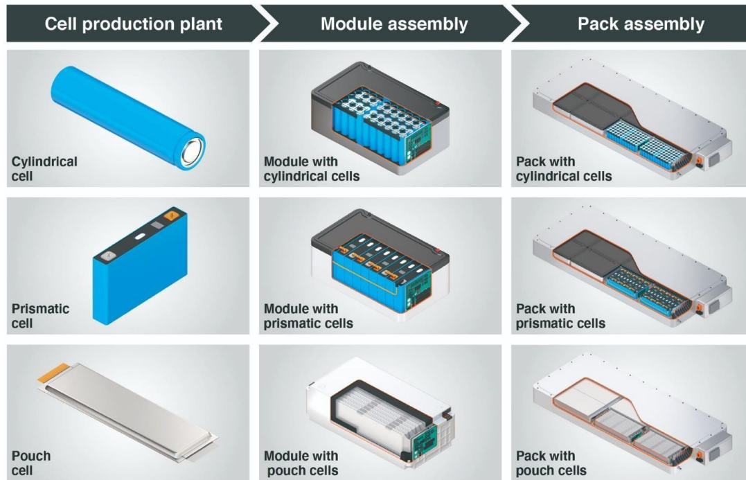
Figure 21: Battery components
