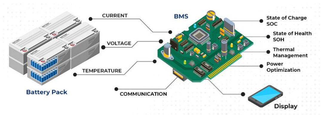
Figure 7: BMS
