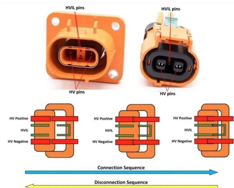
Figure 28: HVIL pins
