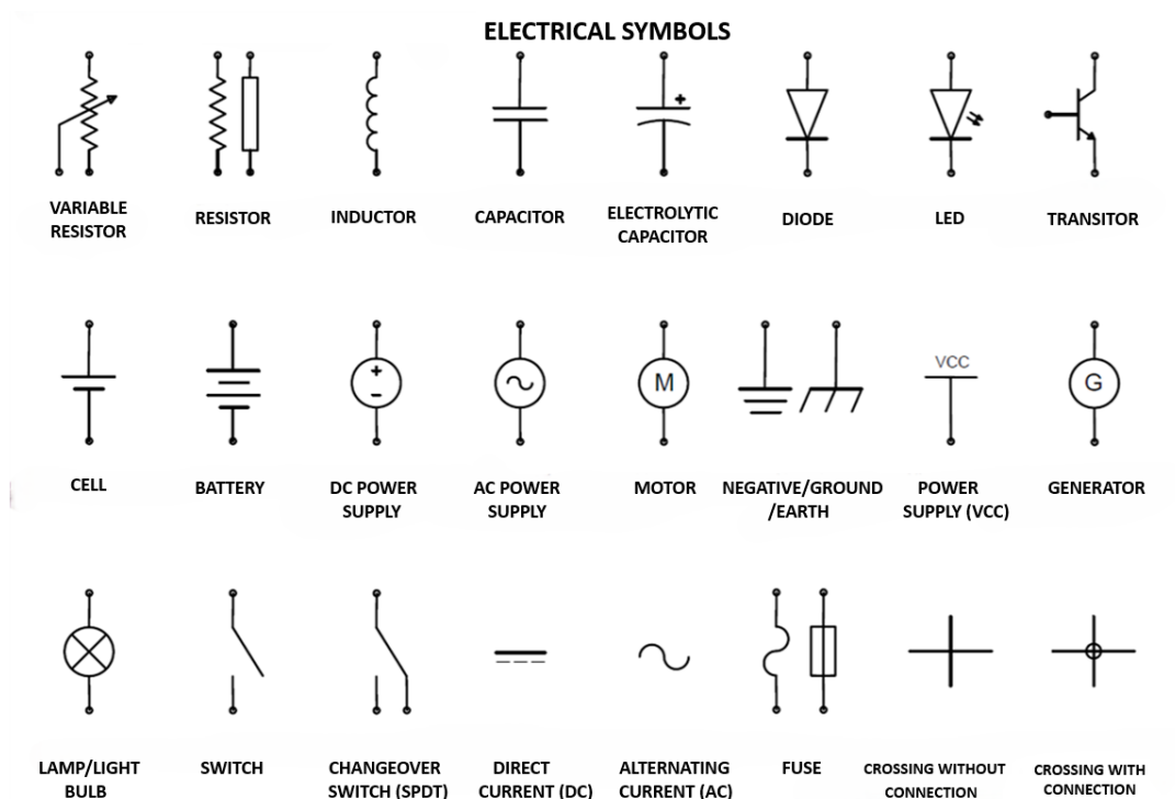
Figure 12: Electrical Symbols
